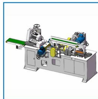
轻型车片专用组合磨床 Light vehicle combined grinder
