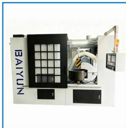
立卧数控外弧磨床 Vertical and horizontal CNC outside grinder
