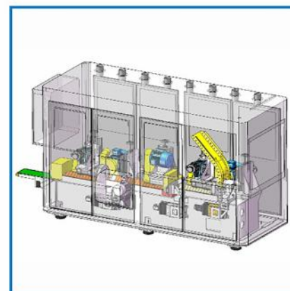
轻型车组合磨床 Combined grinder for light vehicles
