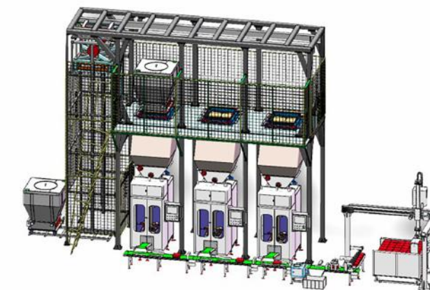
自动上料称量装袋系统 Automatic feeding and weighing and bagging system
